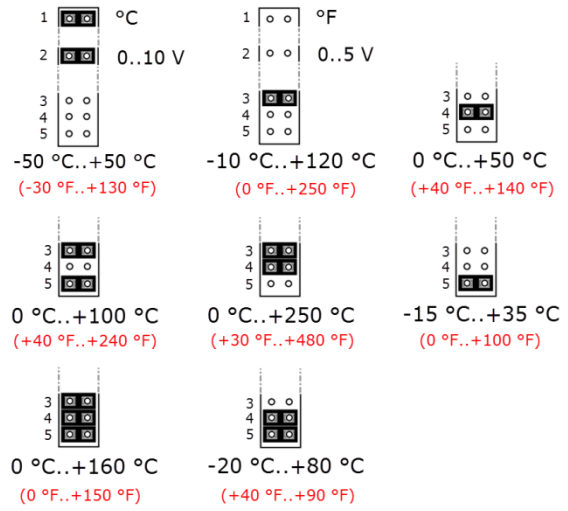
fig. (Measuring range and offset adjustment, default settings: -20 °C..+80 °C | 0 K)
